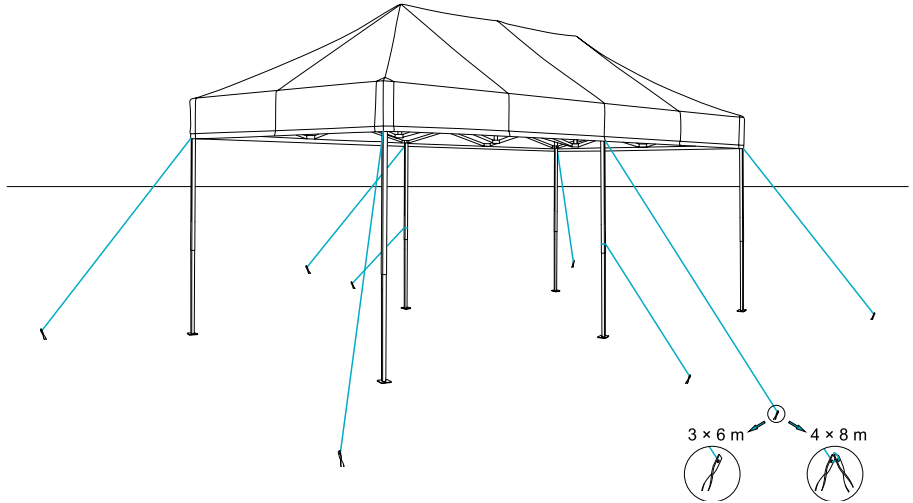
Fig. 1. Mitkotent Premium 3 × 6 m and Octa Pro 4 × 8 m tents lines mounting
